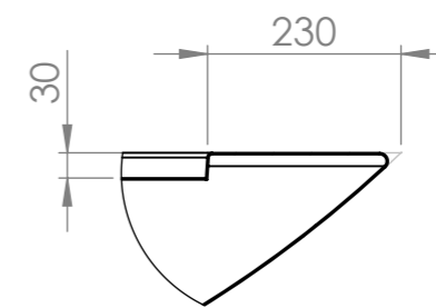
DETAIL C SCALE 1 : 10
